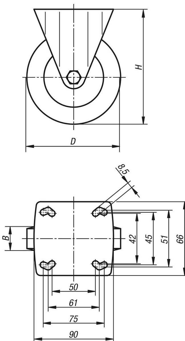
fixed castor
