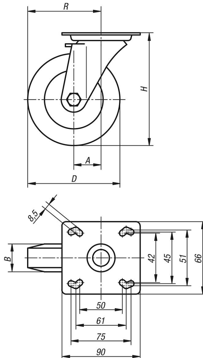
swivel castor
